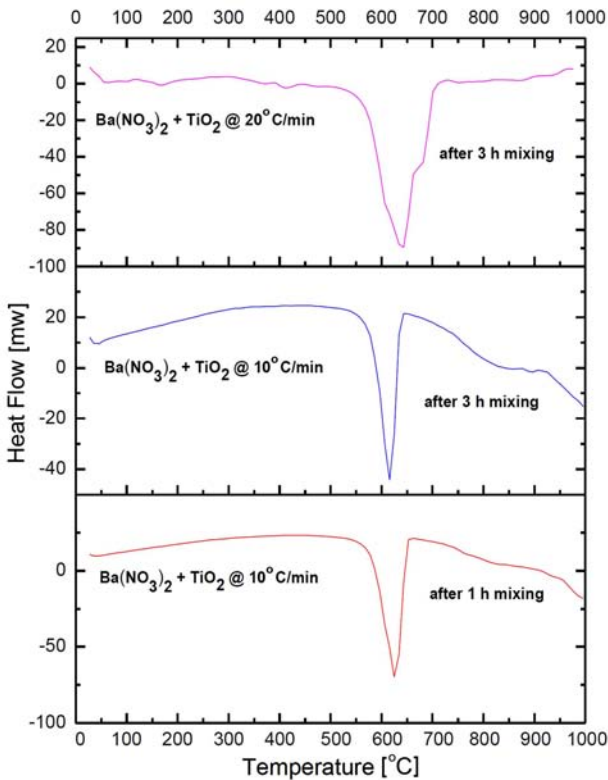
Figure 4. DSC curves (obtained with different heating rates) of the mixture of \text{Ba}(\text{NO}_3)_2 + \text{TiO}_2 prepared by different mixing times
