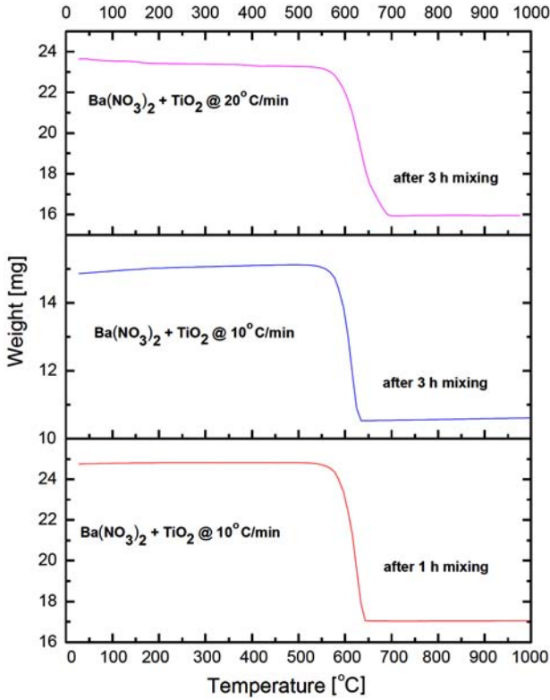
Figure 3. TG curves (obtained with different heating rates) of the mixture of \text{Ba}(\text{NO}_3)_2 + \text{TiO}_2 prepared by different mixing times
