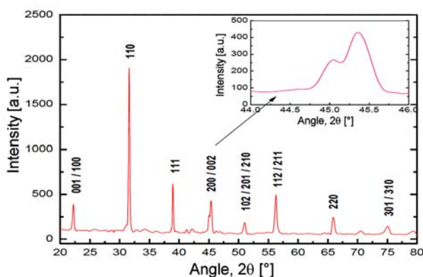
Figure 6. X-ray diffraction pattern of synthesized BaTiO 3 powder
