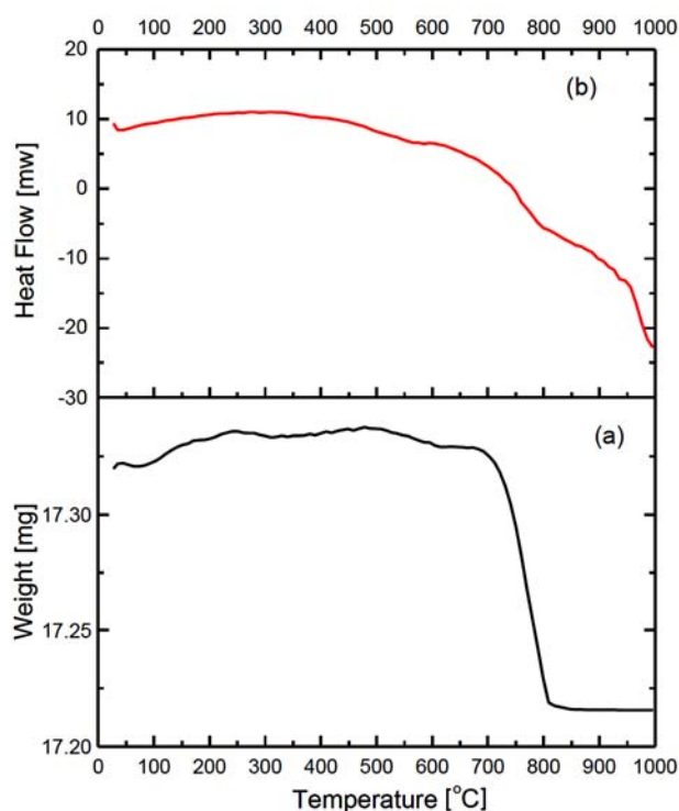
Figure 5. TG (a) and DSC curve (b) of synthesized BaTiO 3 powder
