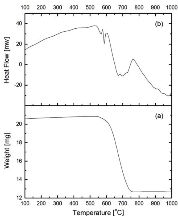
Figure 2. TG (a) and DSC curves (b) of \text{Ba}(\text{NO}_3)_2
