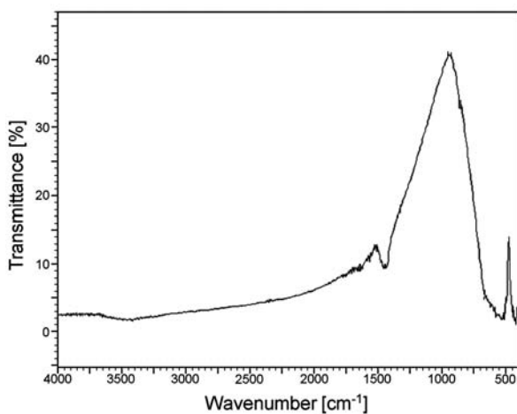
Figure 7. FTIR spectrum of synthesized BaTiO 3 powder
