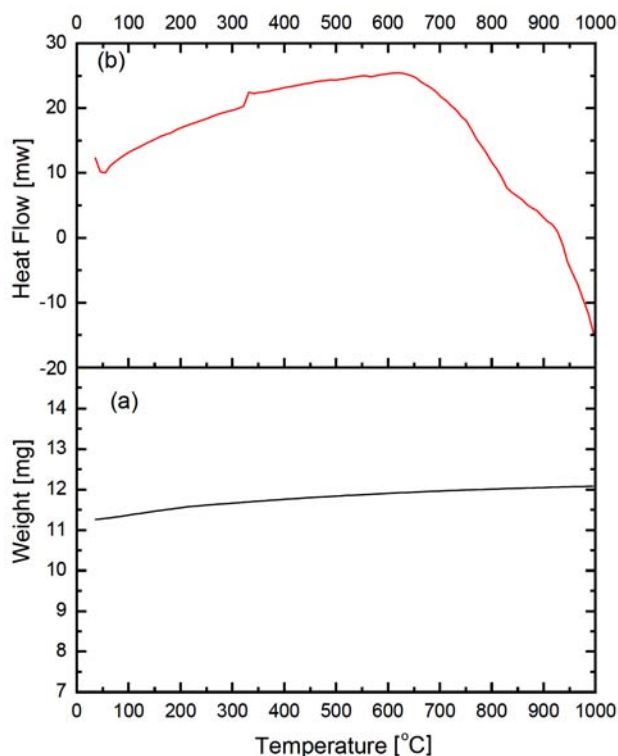
Figure 1. TG (a) and DSC curves (b) of \text{TiO}_2
