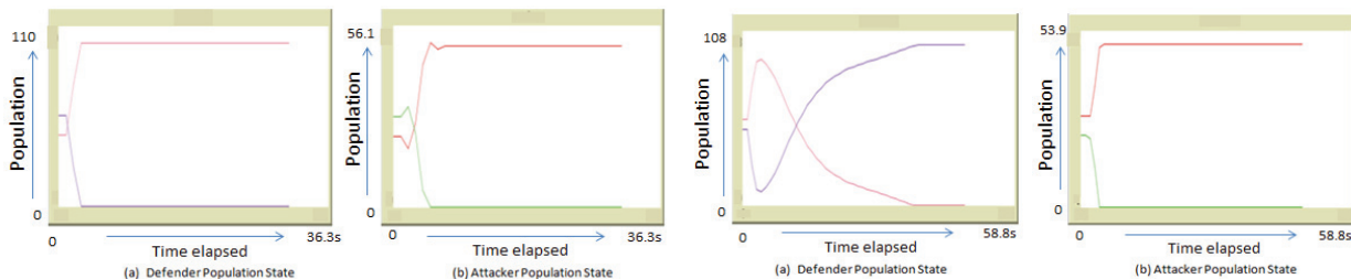
Fig. 5: Population State when (M_1, M_2) = (13.2, -8) ESS(1, 1)
