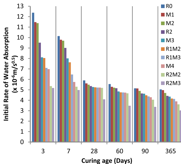
Fig. 6. Graph between Initial Rate of water absorption and days of curing in water.
