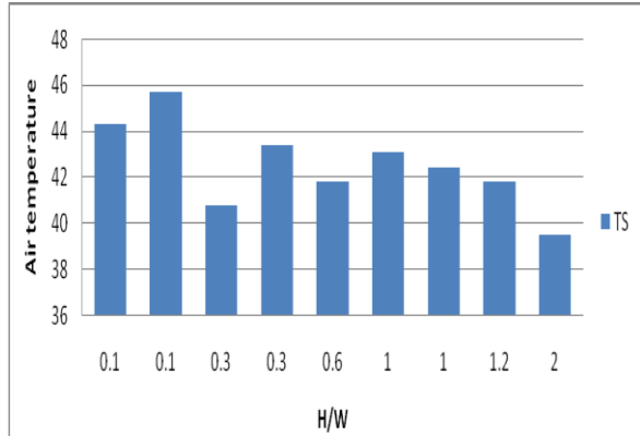
Fig.7 Temperature Variation with H/W ratio.
