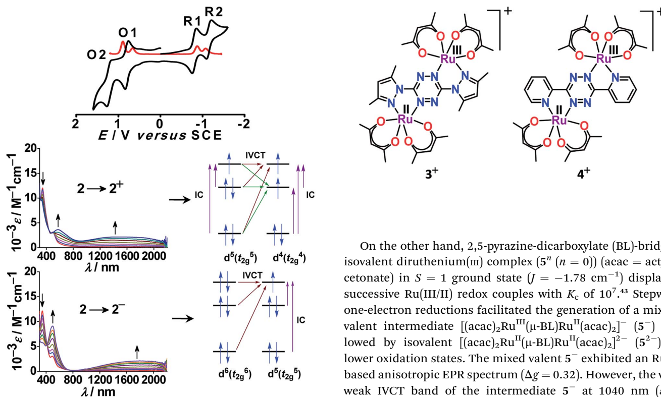
Fig. 5 Cyclic (black) and differential pulse (red) voltammograms of 2 in CH 3 CN (top). UV-vis-NIR spectroelectrochemistry in CH 3 CN and the sketch for IVCT and IC transitions (bottom).
