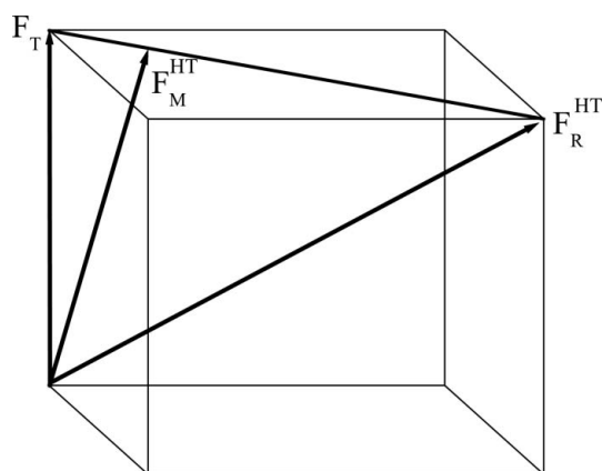
Figure 8 Direction of polarization vector in the F_R^{HT} [111], F_M^{HT} [in the plane ( \bar{1}\bar{1}0 )] and F_T [001] phases of PZT.
