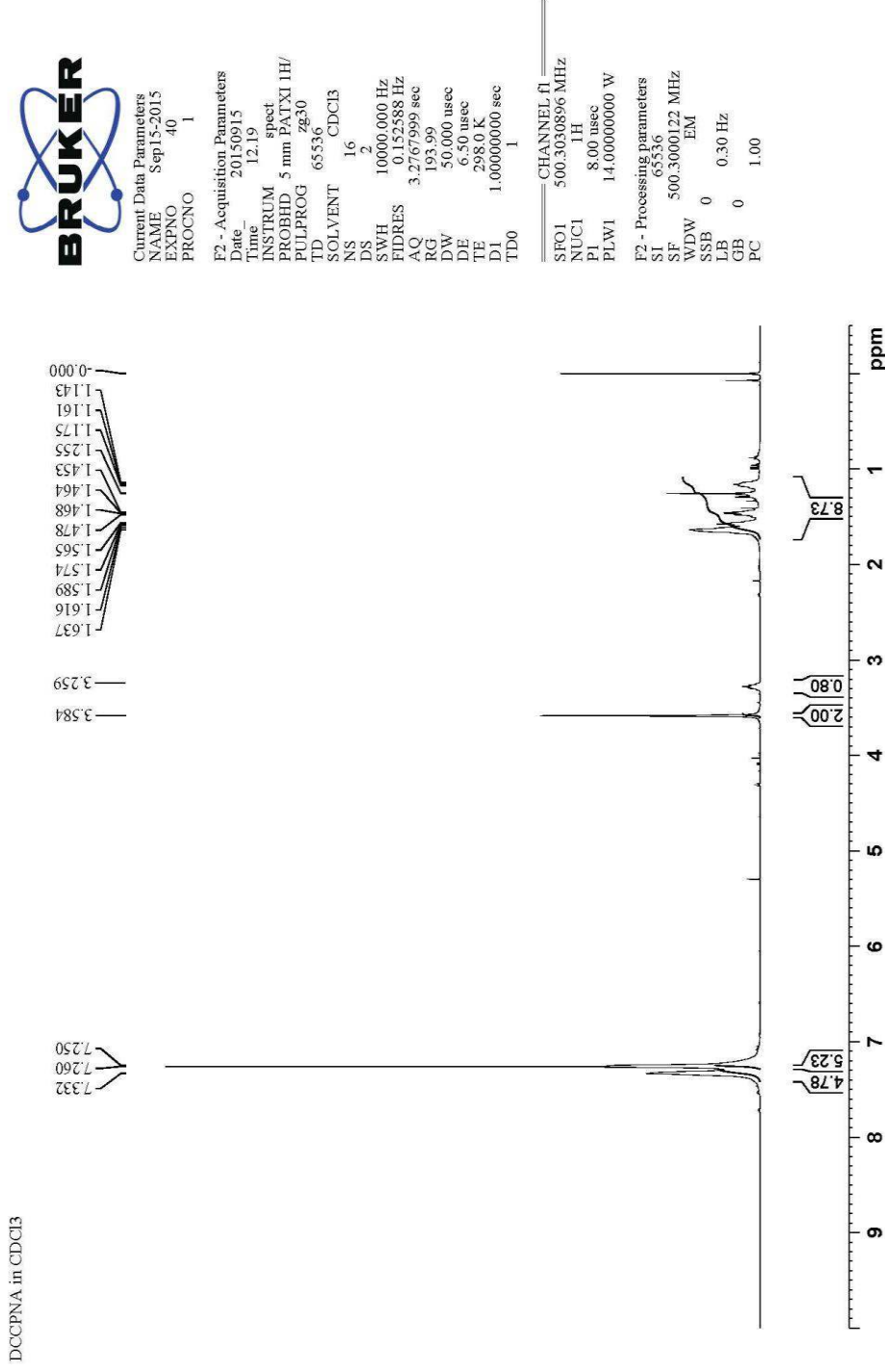
1 H NMR spectrum of 2-Cyclopentylamino-N,N-diphenyl-acetamide (S9)
