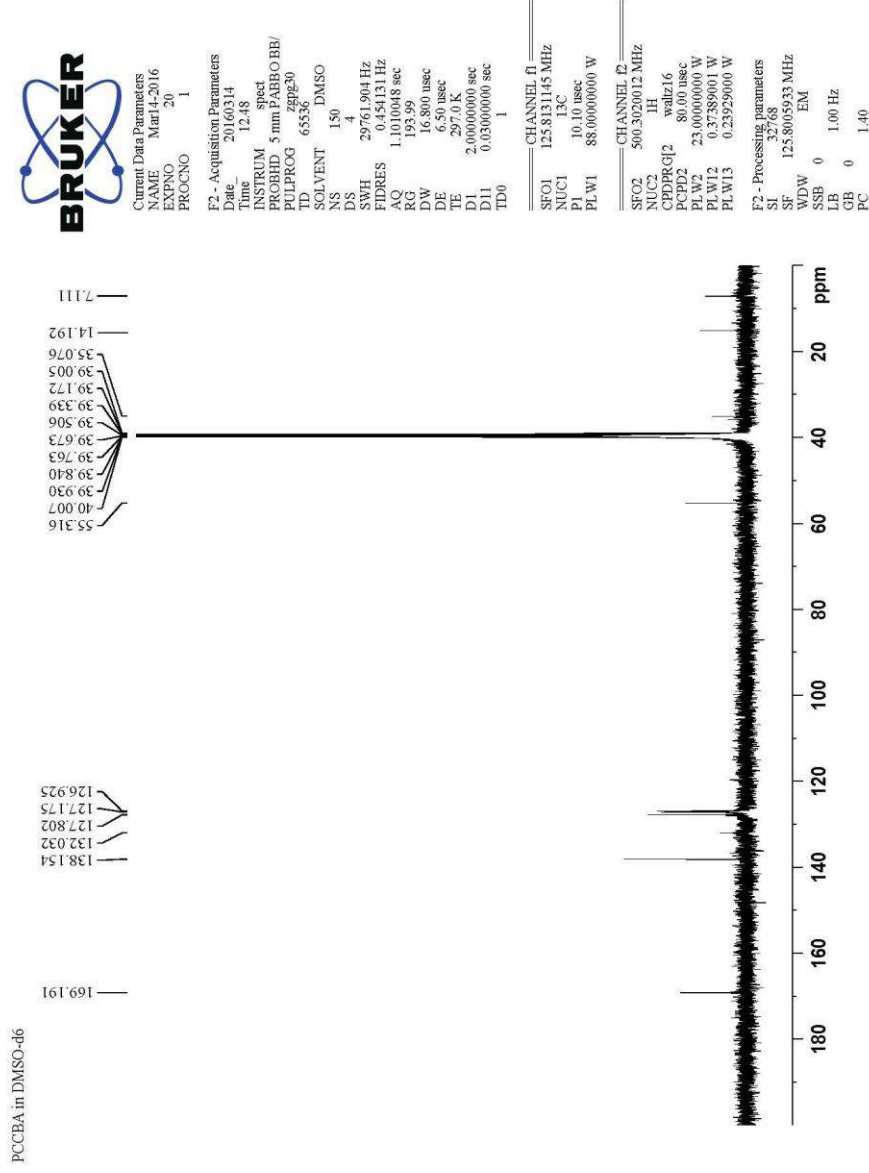
13 C NMR spectrum of 2-(cyclobutylamino)-1-(10H-phenothiazin-10-yl)ethan-1-one (S2)
