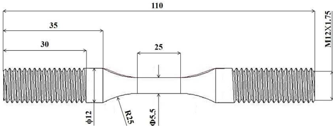
FIGURE 2.4: Schematic of the cylindrical LCF specimen with dimensions in mm.
