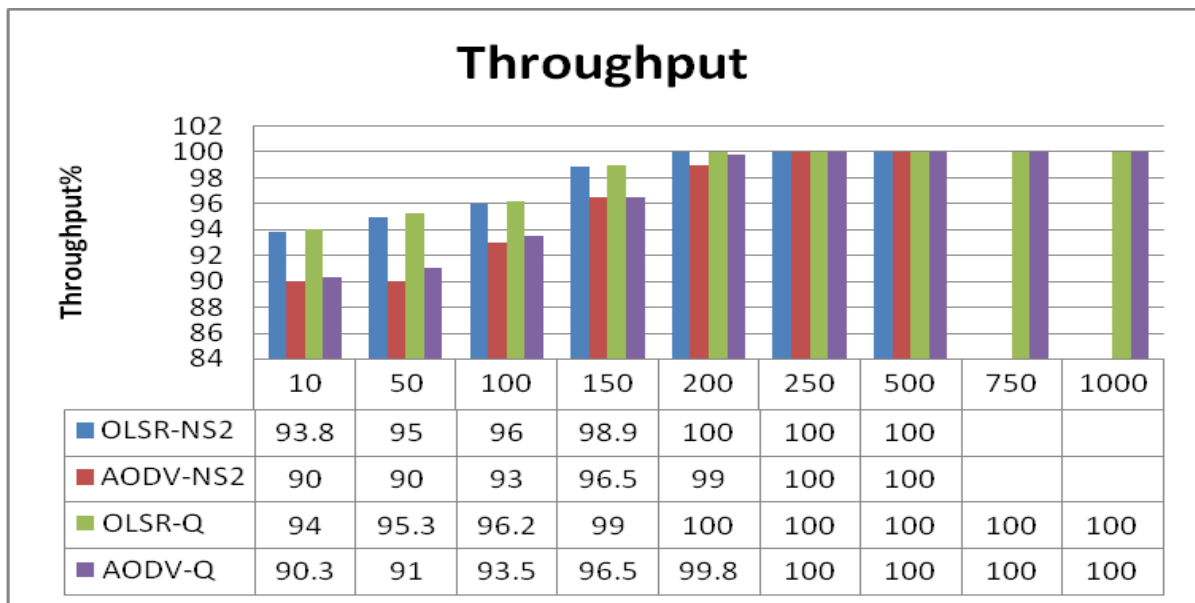
Figure 3.10: Throughput under variable node density
