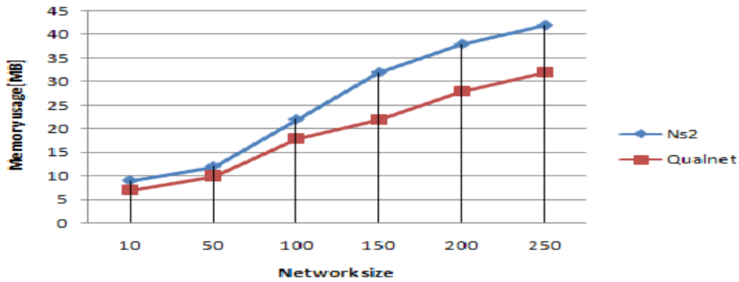
Figure 3.8: Memory usage performance with nodes increment & simulation area 250x250
