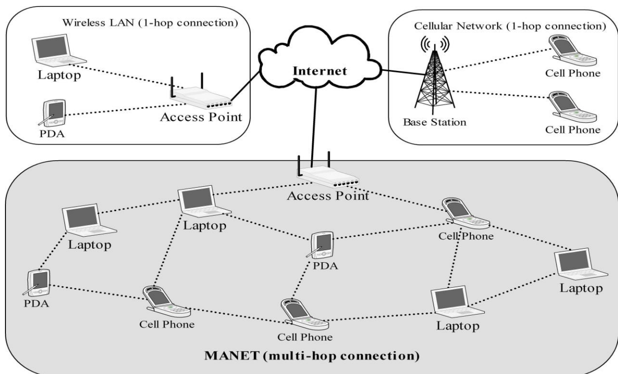
Figure 1.2: Mobile ad hoc network
