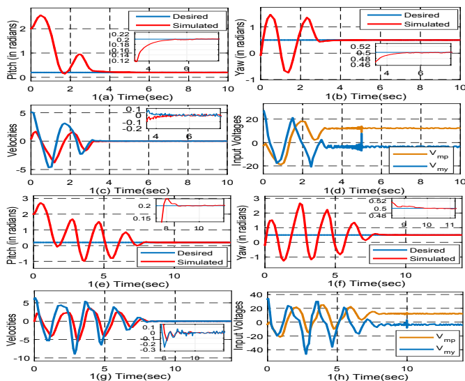
Fig. 1. States and input voltages of system (22) in predefined time t_a = 5 sec (1(a)(b)(c)(d)) and 10 sec (1(e)(f)(g)(h))
