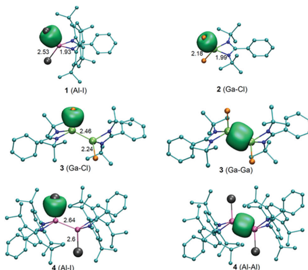
Fig. 5 The optimized geometries of 1 , 2 , 3 , and 4 were obtained at the B3LYP/ECP(I),6-311+G** level of theory and the \sigma -type NBOs (isosurface = 0.06 a.u.) of the Ga–Cl, Al–I, Ga–Ga, and Al–Al bonds in these compounds. The hydrogen atoms are not shown for clarity. The important bond distances are indicated in Å units.
