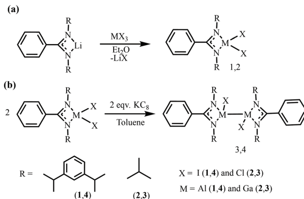
Scheme 1 Synthetic route for the synthesis of compounds 1–4.
