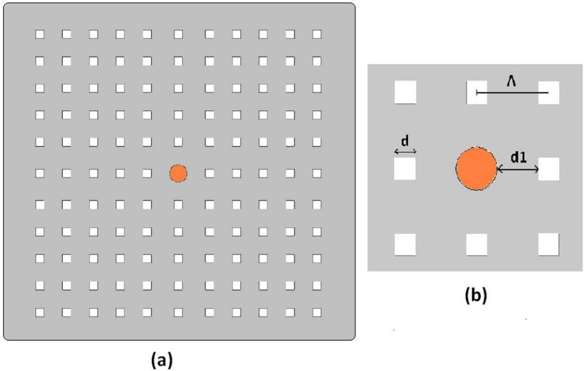
Figure 5.1 Transverse cross-section of the (a) Designed PCF with 5 air-hole rings around a solid circular core. (b) Inner core with first air hole ring showing pitch \Lambda , square hole width d and distance between first ring and core as d^1 .
