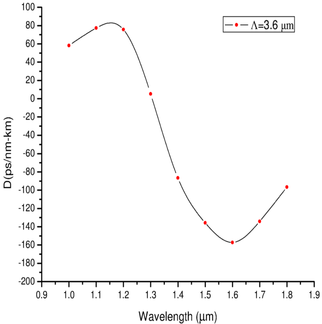
Figure 5.3 Dispersion properties of the PCF with \Lambda=3.6 \mu\text{m} .
