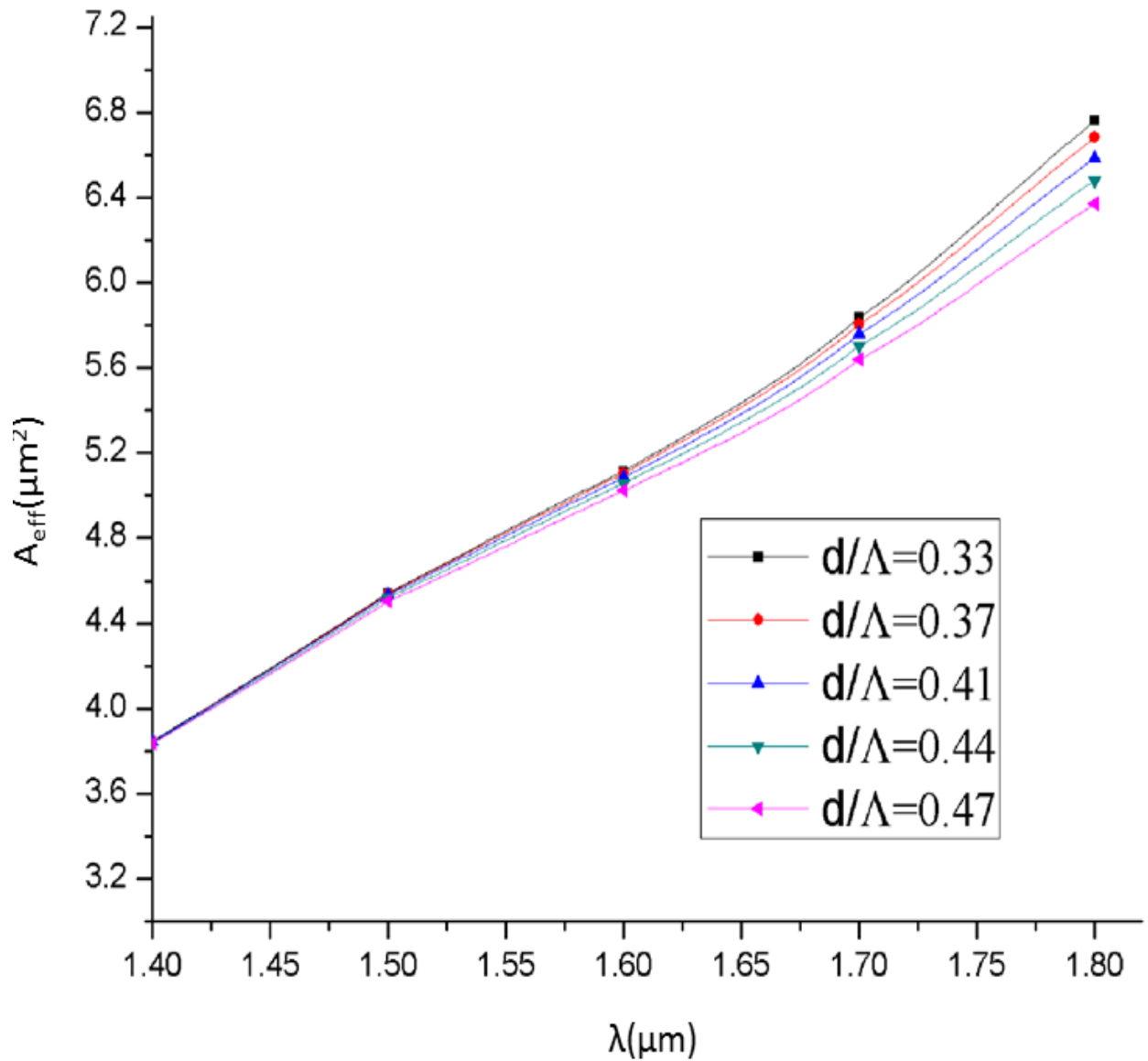
Figure 5.6 Variation of effective mode area with wavelength.
