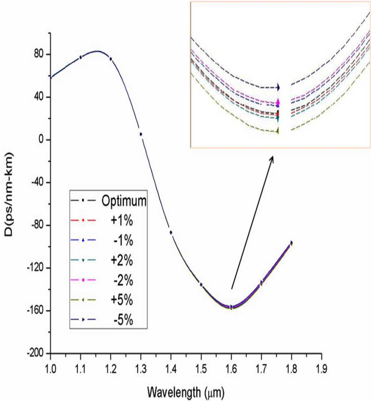
Figure 5.5 Dispersion properties of PCF: Values of D calculated at d^1 , \pm 1 - 5\% variation in d^1 and plotted against wavelength. Inset shows zoom image of the specific graph portion situated at the starting point of arrow.
