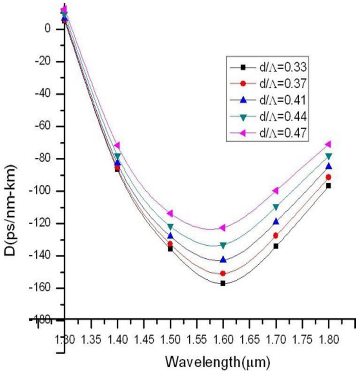
Figure 5.4 Dispersion properties of the PCF with different values of d/\Lambda keeping square hole width d=1.2\mu\text{m} as constant.
