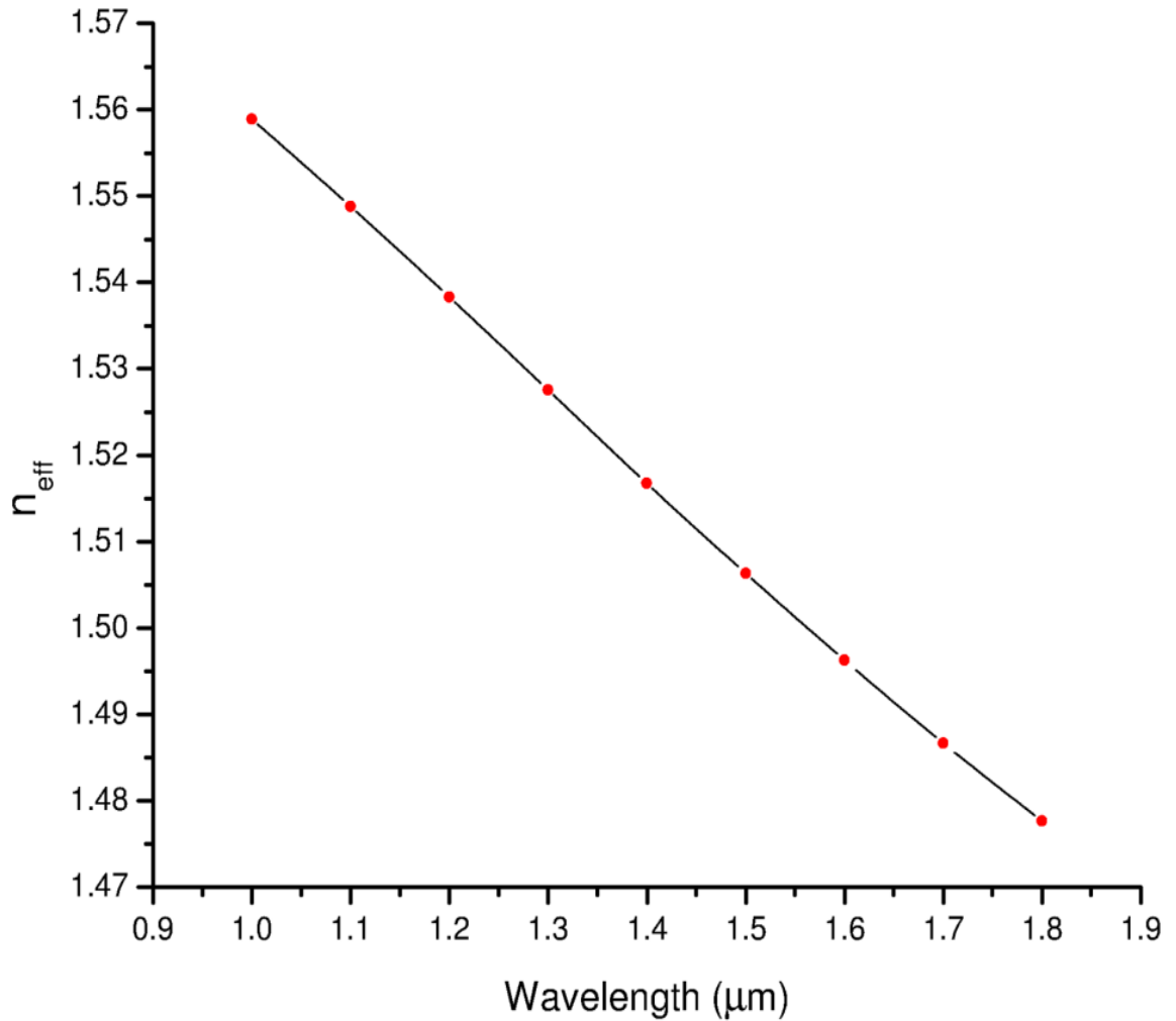
Figure 5.2 Effective refractive index of the PCF with \Lambda=3.6 \mu\text{m} plotted against wavelength.
