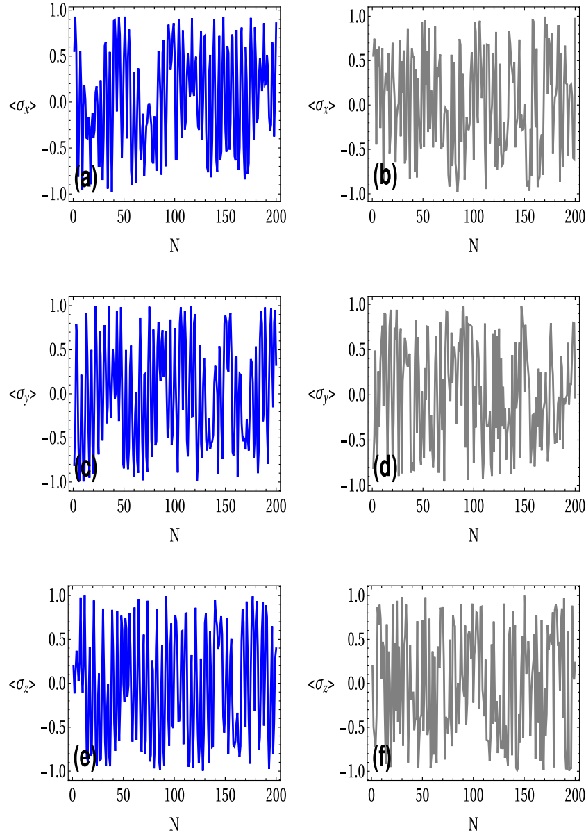
Fig. 4. Spin dynamics for \langle \sigma_x \rangle , \langle \sigma_y \rangle and \langle \sigma_z \rangle in the regular regime at K = 0.5 (see (a), (c) and (e)) and \langle \sigma_x \rangle , \langle \sigma_y \rangle and \langle \sigma_z \rangle in the chaotic regime at K = 10 (see (b), (d) and (f)). The parameters are m = 1 , g = 1 , \omega_0 = 1 , \omega_r = 0.2 , T = 1 , \alpha = \pi/2 . The values of the parameters in the real units: K = \epsilon I_0 T \frac{6\pi\mu}{m^2\omega_r^2} , \mu = \frac{\omega_r^2 m}{2\alpha_0^2} , I_0 = \frac{m}{2}\chi_0^2\omega_r , m = 6 \times 10^{-17} Kg, x_0 = a_0 = 5 \times 10^{-3} m, T = 10\mu\text{s} , \omega_r = \omega_0 = 2\pi \times 5 \times 10^6 Hz, for chaotic \epsilon = 0.003 and for regular \epsilon = 0.0003 .
