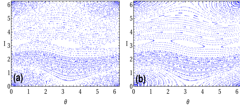
Fig. 13. The Phase space plot of cantilever's dynamics constructed through the recurrence relations equation (37) with feedback in (a) and (b) the regular regime K = 0.5 (Blue) where the phase space is covered by two different phase trajectories: open hyperbolic and some part of closed ellipse. The parameters for Fig. 13(a) are m = 1, g = 0.1, \omega_0 = 10, \omega_r = 0.2, T = 1 . The parameters for Fig. 13(b) are m = 1, g = 0.01, \omega_0 = 1, \omega_r = 0.2, T = 1 . The values of the parameters in the real units: K = \epsilon I_0 T \frac{6\pi\mu}{m^2\omega_r^2}, \mu = \frac{\omega_r^2 m}{2a_0^2}, I_0 = \frac{m}{2} x_0^2 \omega_r, m = 6 \times 10^{-17} Kg, x_0 = a_0 = 5 \times 10^{-3} m, T = 10\mu\text{s}, \omega_r = \omega_0 = 2\pi \times 5 \times 10^6 Hz, for the regular case \epsilon = 0.0003 .
