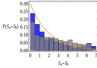
Fig. 7. Histogram plot of level statistics of Hamiltonian \hat{H}_n in the regular regime at K = 0.5 (Blue) and in the chaotic regime K = 10 (Gray). A reference plot for Poissonian statistics (Orange) is also shown. For this plot we have taken up to 1000 kicks to get the ensemble. The parameters are m = 1 , g = 1 , \omega_0 = 1 , \omega_r = 0.2 , T=1 , \alpha = \pi/2 . The values of parameters: K = \epsilon I_0 T \frac{6\pi\mu}{m^2\omega_0^2} , \mu = \frac{\omega_r^2 m}{2a_0^2} , I_0 = \frac{m}{2}\chi_0^2\omega_r , m = 6 \times 10^{-17} Kg, x_0 = a_0 = 5 \times 10^{-3} m, T=10 \mu s, \omega_r = \omega_0 = 2\pi \times 5 \times 10^6 Hz, for chaotic case \epsilon = 0.003 and for the regular case \epsilon = 0.0003 .
