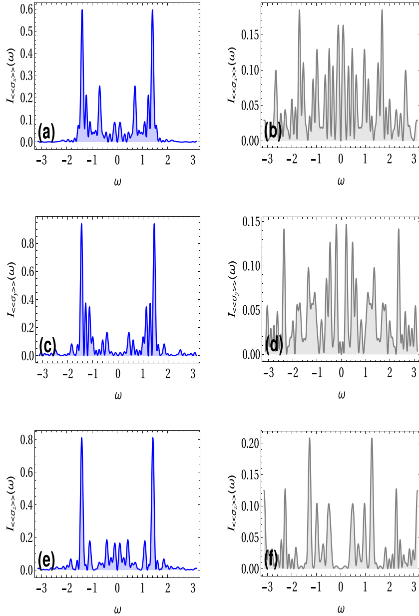
Fig. 12. Statistical average of Fourier Power spectrum density (Spin-1/2 system) for \langle\langle\sigma_x\rangle\rangle , \langle\langle\sigma_y\rangle\rangle and \langle\langle\sigma_z\rangle\rangle in the regular regime ((a), (c) and (e)) at K = 0.5 (Blue), and in the chaotic regime ((b), (d) and (f)) at K = 10 (Gray). For calculating Statistical average of Spin dynamics(Spin-1/2 system) we have taken 15 different sets of (I_0, \theta_0) . The parameters used for the plot are m = 1 , g = 1 , \omega_0 = 1 , \omega_r = 0.2 , T = 1 , \alpha = \pi/2 . The values of the parameters in the real units: K = \epsilon I_0 T \frac{6\pi\mu}{m^2\omega_r^2} , \mu = \frac{\omega_r^2 m}{2\alpha_0^2} , I_0 = \frac{m}{2}\alpha_0^2\omega_r , m = 6 \times 10^{-17} Kg, \alpha_0 = a_0 = 5 \times 10^{-3} m, T = 10\mu\text{s} , \omega_r = \omega_0 = 2\pi \times 5 \times 10^6 Hz, for chaotic case \epsilon = 0.003 and for the regular case \epsilon = 0.0003 .
