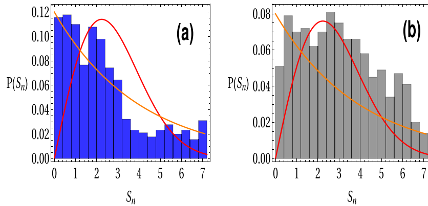
Fig. 10. Histogram plot of level statistics of Hamiltonian \hat{H}_n = \hat{H}_{NV} + g\hat{V}_{c,NV} for spin-1 system (a) in the regular regime at K = 0.5 (Blue) and (b) in the chaotic regime K = 10 (Gray). A reference plot for Poissonian statistics (Orange) and Gaussian statistics (Red) is also shown. 1000 kicks are considered. The parameters are m = 1 , g = 1 , \Omega = 1 , \delta = 1 , \omega_r = 0.2 , T=1 , \alpha = \pi/2 . The values of parameters: K = \epsilon I_0 T \frac{6\pi\mu}{m^2\omega_0^2} , \mu = \frac{\omega_r^2 m}{2a_0^2} , I_0 = \frac{m}{2} x_0^2 \omega_r , m = 6 \times 10^{-17} Kg, x_0 = a_0 = 5 \times 10^{-3} m, T=10 \mu\text{s} , \omega_r = \omega_0 = 2\pi \times 5 \times 10^6 Hz, for chaotic case \epsilon = 0.003 and for the regular case \epsilon = 0.0003 .
