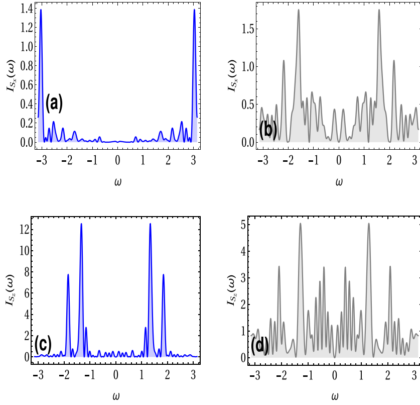
Fig. 8. Fourier Power spectrum density for the components S_{x,z} in the regular regime ((a) and (c)) at K = 0.5 (Blue), and in the chaotic regime ((b) and (d)) at K = 10 (Gray). The parameters used for the plot are m = 1 , g = 1 , \Omega = 1 , \delta = 1 , \omega_r = 0.2 , T = 1 , \alpha = \pi/2 . The values of the parameters in the real units: K = \epsilon I_0 T \frac{6\pi\mu}{m^2\omega_r^2} , \mu = \frac{\omega_r^2 m}{2a_0^2} , I_0 = \frac{m}{2} x_0^2 \omega_r , m = 6 \times 10^{-17} Kg, x_0 = a_0 = 5 \times 10^{-3} m, T = 10\mu\text{s} , \omega_r = \omega_0 = 2\pi \times 5 \times 10^6 Hz, for chaotic case \epsilon = 0.003 and for the regular case \epsilon = 0.0003 .
