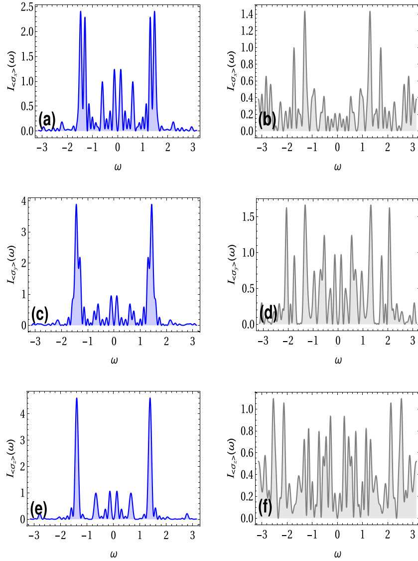
Fig. 3. Fourier Power spectrum density for expectation values of \sigma_{x,y,z} in the regular regime ((a), (c) and (e)) at K = 0.5 (Blue), and in the chaotic regime ((b), (d) and (f)) at K = 10 (Gray). The parameters used for the plot are m = 1 , g = 1 , \omega_0 = 1 , \omega_r = 0.2 , T = 1 , \alpha = \pi/2 . The values of the parameters in the real units: K = \epsilon I_0 T \frac{6\pi\mu}{m^2\omega_r^2} , \mu = \frac{\omega_r^2 m}{2u_0^2} , I_0 = \frac{m}{2} x_0^2 \omega_r , m = 6 \times 10^{-17} Kg, x_0 = a_0 = 5 \times 10^{-3} m, T = 10 \mu s, \omega_r = \omega_0 = 2\pi \times 5 \times 10^6 Hz, for chaotic case \epsilon = 0.003 and for the regular case \epsilon = 0.0003 .
