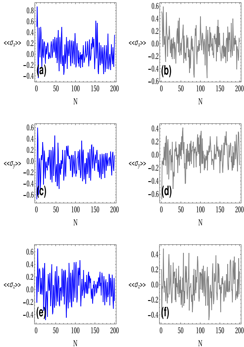
Fig. 11. Statistical average of spin dynamics (Spin-1/2 system) for \langle\langle\sigma_x\rangle\rangle , \langle\langle\sigma_y\rangle\rangle and \langle\langle\sigma_z\rangle\rangle in the regular regime at K = 0.5 ((a), (c) and (e)) and in the chaotic regime at K = 10 ((b), (d) and (f)). For calculating statistical average of spin dynamics (Spin-1/2 system) we have taken 15 different sets of (I_0, \theta_0) . The parameters are m = 1 , g = 1 , \omega_0 = 1 , \omega_r = 0.2 , T = 1 , \alpha = \pi/2 . The values of the parameters in the real units: K = \epsilon I_0 T \frac{6\pi\mu}{m^2\omega_r^2} , \mu = \frac{\omega_0^2 m}{2a_0^2} , I_0 = \frac{m}{2} x_0^2 \omega_r , m = 6 \times 10^{-17} Kg, x_0 = a_0 = 5 \times 10^{-3} m, T = 10\mu\text{s} , \omega_r = \omega_0 = 2\pi \times 5 \times 10^6 Hz, for chaotic \epsilon = 0.003 and for regular \epsilon = 0.0003 .
