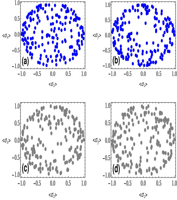
Fig. 2. Poincaré sections for (\langle \sigma_x \rangle, \langle \sigma_z \rangle) and (\langle \sigma_y \rangle, \langle \sigma_z \rangle) in the regular regime at K = 0.5 ((a) and (b)) and chaotic regime at K = 10 ((c) and (d)). The parameters are m = 1 , g = 1 , \omega_0 = 1 , \omega_r = 0.2 , T = 1 , \alpha = \pi/2 . The values of the parameters in the real units are K = \epsilon I_0 T \frac{6\pi\mu}{m^2\omega_r^2} , \mu = \frac{\omega_r^2 m}{2\omega_0^2} , I_0 = \frac{m}{2}\chi_0^2\omega_r , m = 6 \times 10^{-17} Kg, x_0 = a_0 = 5 \times 10^{-3} m, T = 10\mu\text{s} , \omega_r = \omega_0 = 2\pi \times 5 \times 10^6 Hz, for chaotic case \epsilon = 0.003 and for the regular case \epsilon = 0.0003 .
