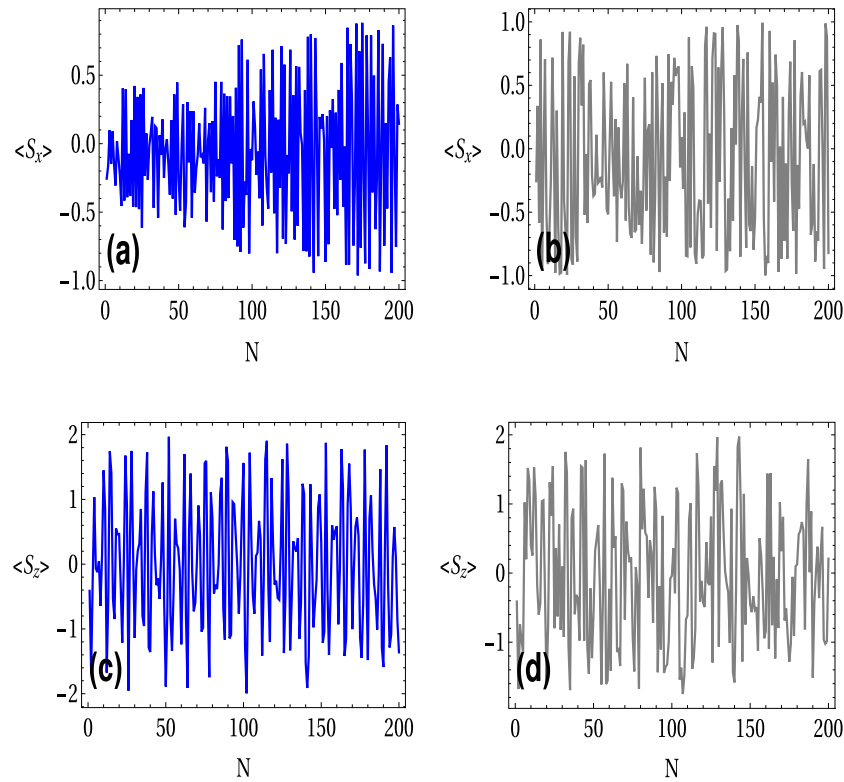
Fig. 9. Spin dynamics for the components S_x and S_z for Spin-1 case in the regular regime at K = 0.5 ((a) and (c)) and in the chaotic regime at K = 10 ((b) and (d)). The parameters are m = 1 , g = 1 , \Omega = 1 , \delta = 1 , \omega_r = 0.2 , T = 1 , \alpha = \pi/2 . The values of the parameters in the real units: K = \epsilon I_0 T \frac{6\pi\mu}{m^2\omega_0^2} , \mu = \frac{\omega_r^2 m}{2a_0^2} , I_0 = \frac{m}{2} x_0^2 \omega_r , m = 6 \times 10^{-17} Kg, x_0 = a_0 = 5 \times 10^{-3} m, T = 10\mu\text{s} , \omega_r = \omega_0 = 2\pi \times 5 \times 10^6 Hz, for chaotic \epsilon = 0.003 and for regular \epsilon = 0.0003 .
