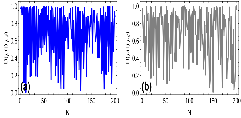
Fig. 5. The quantum coherence in (a) the regular regime at K = 0.5 (Blue) and (b) the chaotic regime at K = 10 (Gray), for the following values of the parameters m = 1, g = 1, \omega_0 = 1, \omega_r = 0.2, T = 1, \alpha = \pi/2 . The values of parameters are K = \epsilon I_0 T \frac{6\pi\mu}{m^2\omega_r^2}, \mu = \frac{\omega_r^2 m}{2a_0^2}, I_0 = \frac{m}{2} x_0^2 \omega_r, m = 6 \times 10^{-17} Kg, x_0 = a_0 = 5 \times 10^{-3} m, T=10 \mu s, \omega_r = \omega_0 = 2\pi \times 5 \times 10^6 Hz, for chaotic \epsilon = 0.003 and for regular \epsilon = 0.0003 .
