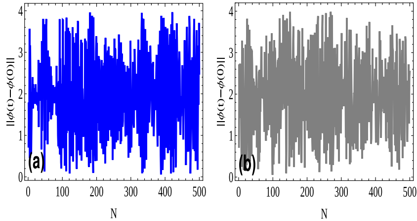
Fig. 6. Quantum Poincaré recurrence as a function of time (i.e. number of kicks) in (a) the regular regime at K = 0.5 (Blue) and (b) the chaotic regime at K = 10 (Gray). The parameters are m = 1, g = 1, \omega_0 = 1, \omega_r = 0.2, T = 1, \alpha = \pi/2 . The values of parameters: K = \epsilon I_0 T \frac{6\pi\mu}{m^2\omega_r^2}, \mu = \frac{\omega_r^2 m}{2a_0^2}, I_0 = \frac{m}{2} x_0^2 \omega_r, m = 6 \times 10^{-17} Kg, x_0 = a_0 = 5 \times 10^{-3} m, T=10 \mu s, \omega_r = \omega_0 = 2\pi \times 5 \times 10^6 Hz, for chaotic \epsilon = 0.003 and for regular \epsilon = 0.0003 .
