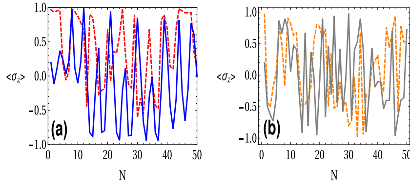
Fig. 14. Spin dynamics with feedback (Solid) and without feedback (Dashed) for \langle \sigma_z \rangle in the regular regime at K = 0.5 (see (a)) and \langle \sigma_z \rangle in the chaotic regime at K = 10 (see (b)). The parameters are m = 1, g = 1, \omega_0 = 1, \omega_r = 0.2, T = 1, \alpha = \pi/2 . The values of the parameters in the real units: K = \epsilon I_0 T \frac{6\pi\mu}{m^2\omega_r^2}, \mu = \frac{\omega_r^2 m}{2a_0^2}, I_0 = \frac{m}{2} x_0^2 \omega_r, m = 6 \times 10^{-17} Kg, x_0 = a_0 = 5 \times 10^{-3} m, T = 10\mu\text{s}, \omega_r = \omega_0 = 2\pi \times 5 \times 10^6 Hz, for chaotic \epsilon = 0.003 and for regular \epsilon = 0.0003 .
