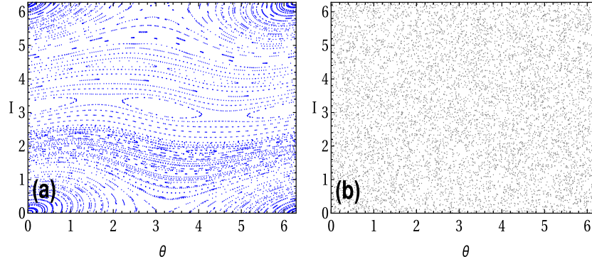
Fig. 1. The Phase space plot of cantilever's dynamics constructed through the recurrence relations equation (6) in (a) the regular regime K = 0.5 (Blue) where the phase space is covered by two different phase trajectories: open hyperbolic and some part of closed elliptic, and (b) the chaotic regime at K = 10 (Gray) where the entire phase space is covered by a chaotic sea. Topologically different phase trajectories are bordered by separatrix line. The values of parameters are: K = \epsilon I_0 T \frac{6\pi\mu}{m^2\omega_r^2} , \mu = \frac{\omega_r^2 m}{2a_0^2} , I_0 = \frac{m}{2}\omega_0^2 x_0 , m = 6 \times 10^{-17} Kg, x_0 = a_0 = 5 \times 10^{-3} m, T = 10 \mu s, \omega_r = \omega_0 = 2\pi \times 5 \times 10^6 Hz, for chaotic case \epsilon = 0.003 and for the regular case \epsilon = 0.0003 .
