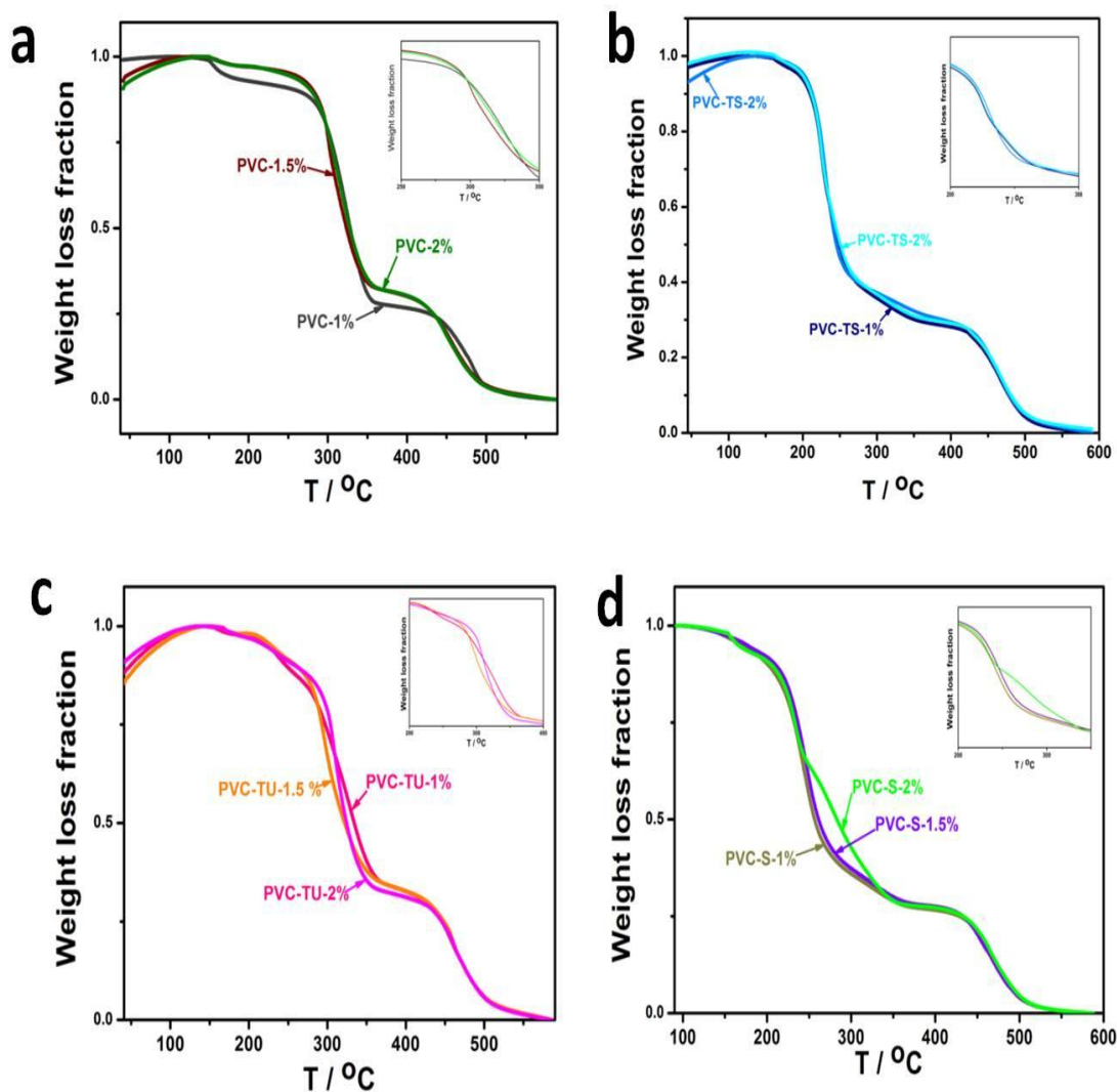
Figure 4.7: Thermograph of polymer composite (a) PVC-1%, PVC-1.5% & PVC-2% (b) PVC-TS-1, PVC-TS-1.5 & PVC-TS-2% (c) PVC-TU-1, 1.5 & 2% (d) PVC-S-1, 1.5 & 2%.
