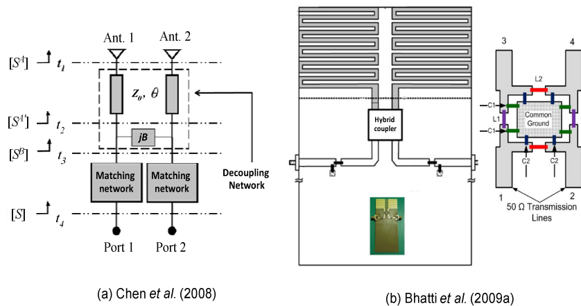
Figure 1.10: External feed network for isolation improvement and (a) Decoupling network, (b) Branch-line decoupling feed network.
