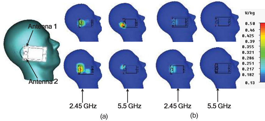
Figure 3.12: Distribution of energy over human head phantom, (a) Average SAR over 1g and (b) Average SAR over 10g.
