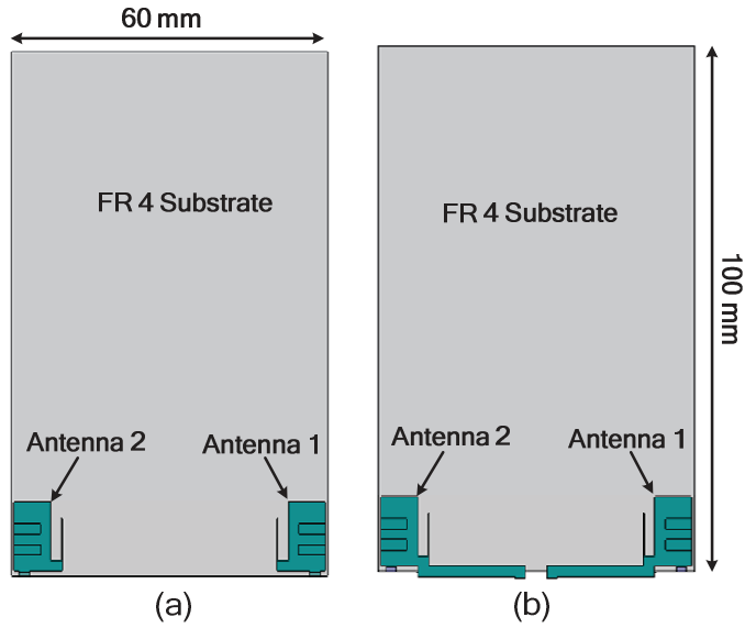
Figure 3.1: Proposed antenna (a) without folded shorting strip, and (b) with folded shorting strip.
