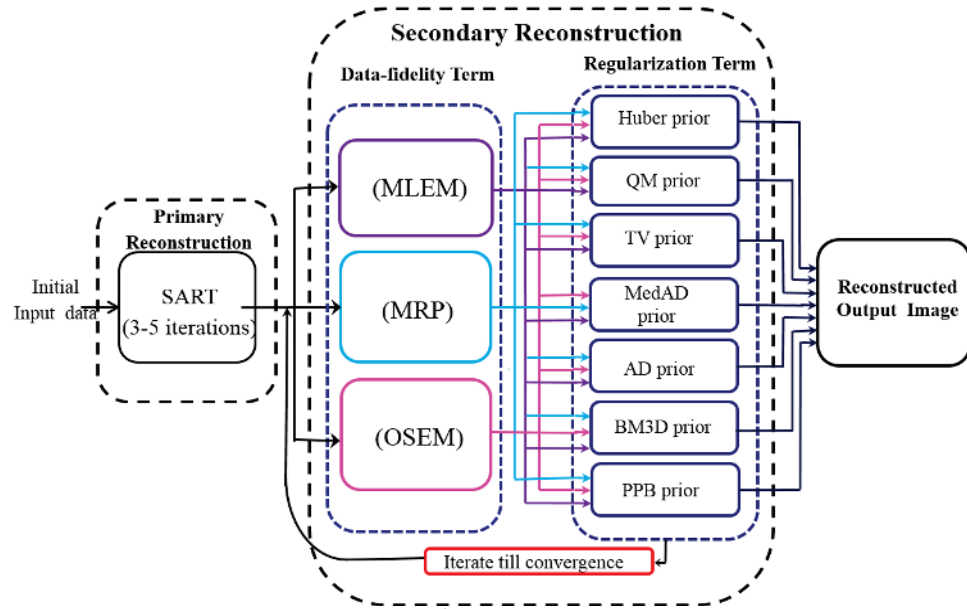
Fig. 4.1: Generalized Hybrid-Cascaded Framework for PET/SPECT Image Reconstruction
