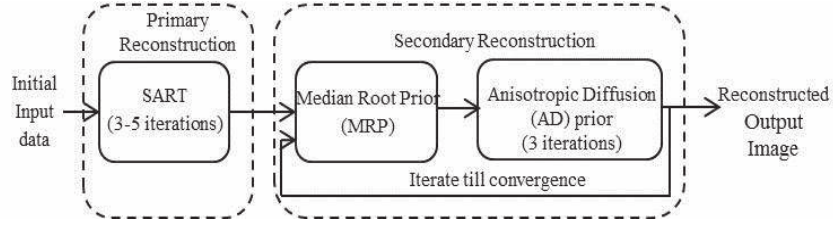
Fig. 4.13: Proposed MRP based hybrid-cascaded framework (Model-2)
