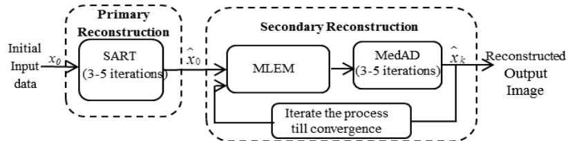
Fig. 4.2: Proposed MLEM based hybrid-cascaded framework (Model-1)
