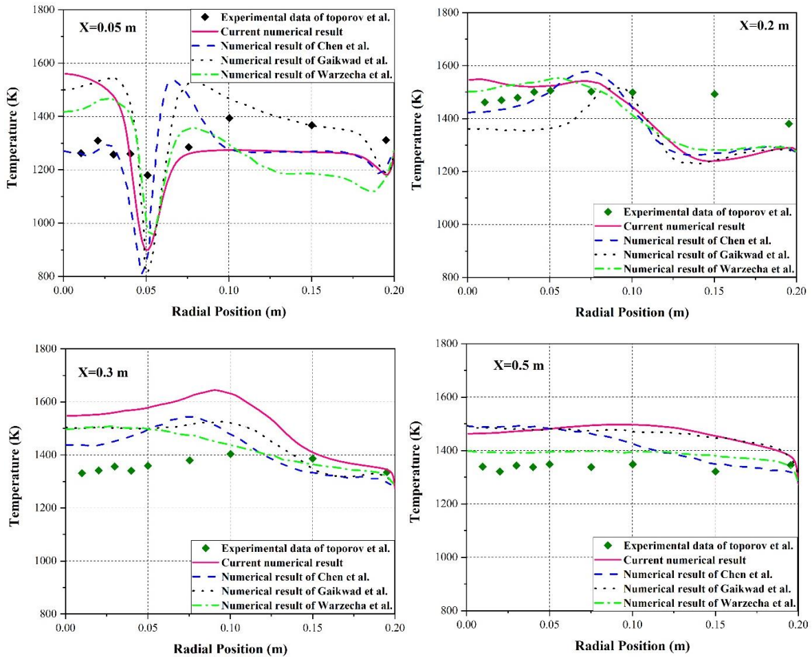
Fig. C2. Comparison of RANS prediction of temperature (K) with RANS prediction of other authors and experimental data at different axial locations from burner
