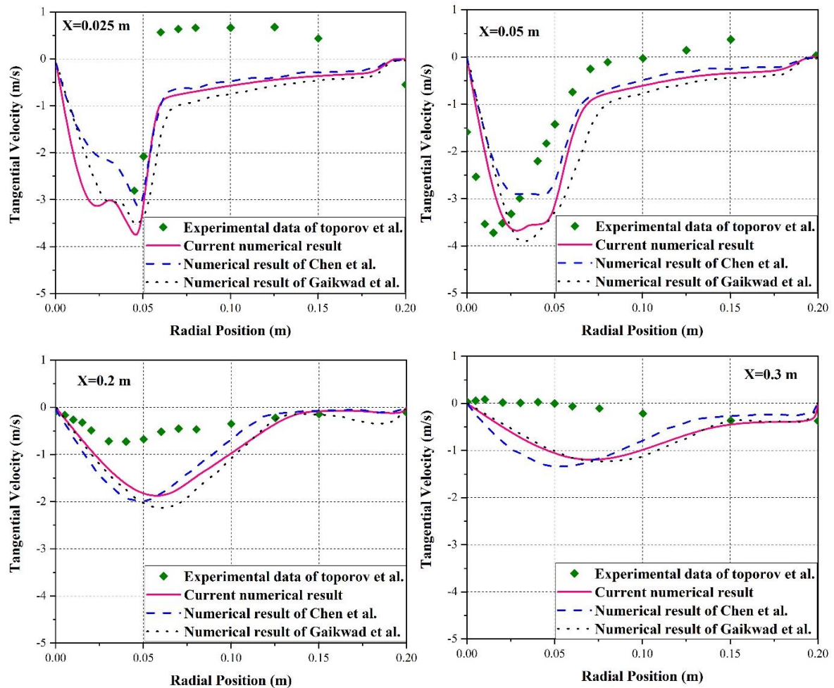
Fig. C1. Comparison of RANS prediction of tangential velocity (m/s) with RANS prediction of other authors and experimental data at different axial locations from burner
