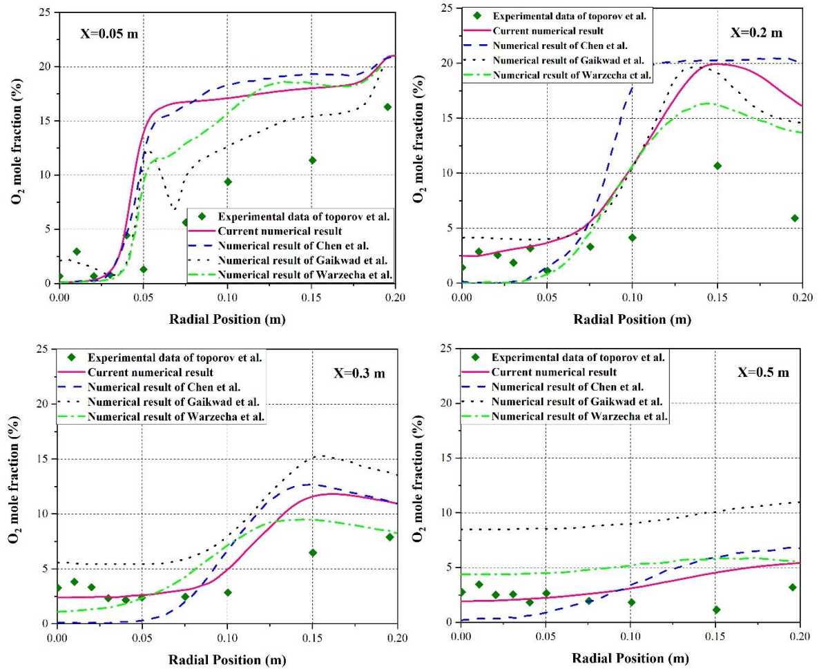
Fig. C3. Comparison of RANS prediction of O 2 mole fraction (%) with RANS prediction of other authors and experimental data at different axial locations from burner
