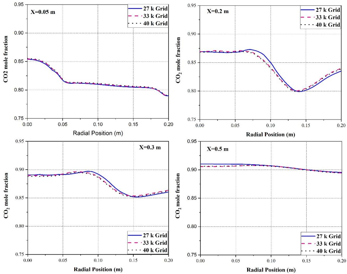
Fig. B4. Radial profile of CO 2 mole fraction at different axial location from burner exit for grid independence test
