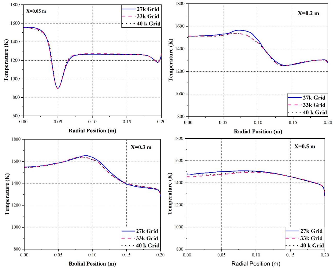
Fig. B2. Radial profile of Temperature (K) at different axial location from burner exit for grid independence test
