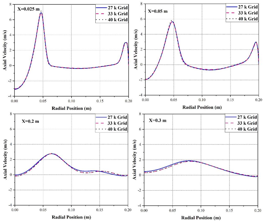
Fig. B1. Radial profile of axial velocity (m/s) at different axial location from burner exit for grid independence test
