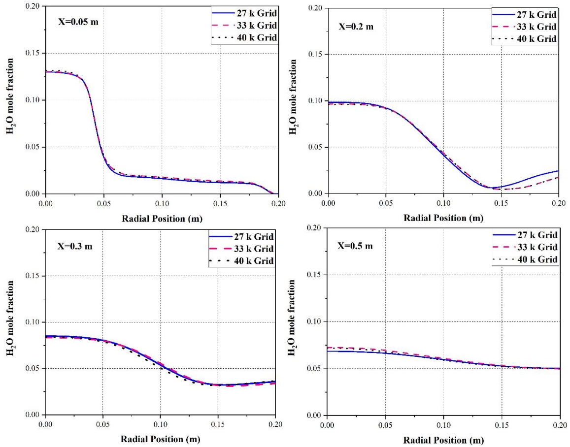
Fig. B5. Radial profile of H 2 O mole fraction at different axial location from burner exit for grid independence test
