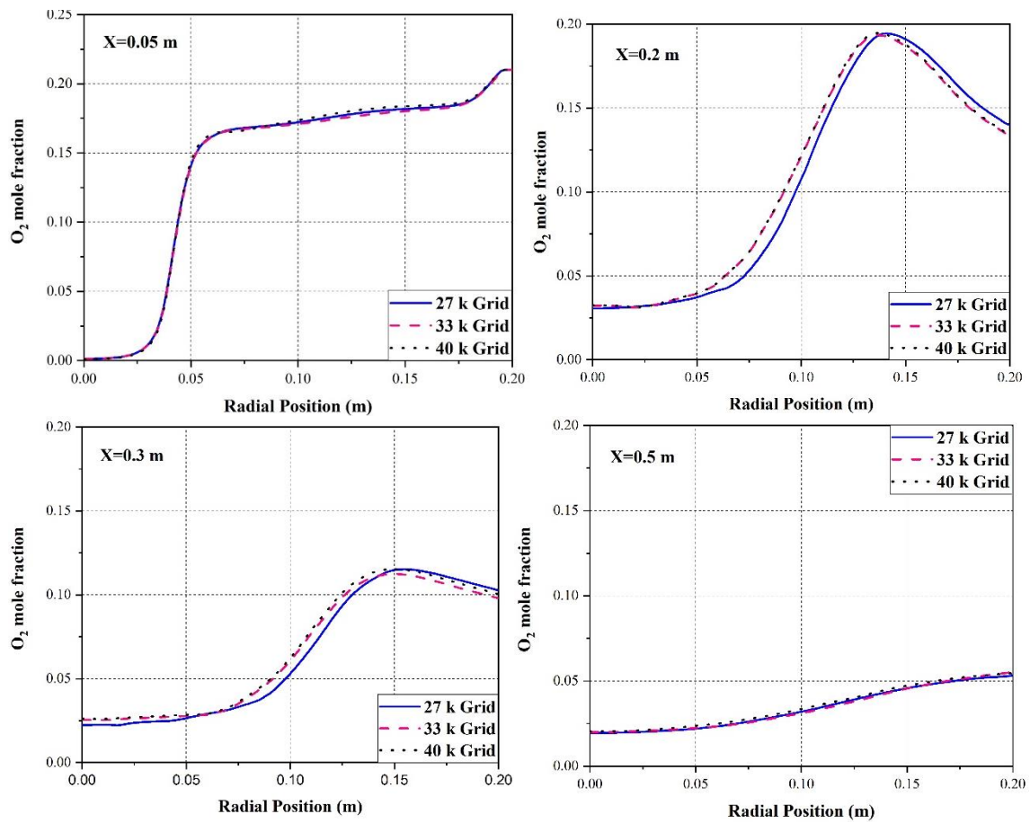
Fig. B3. Radial profile of O 2 mole fraction at different axial location from burner exit for grid independence test
