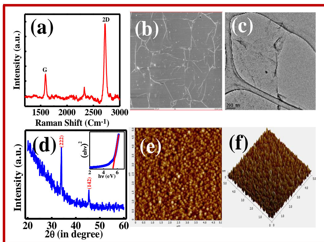
Figure 6.3: a ) Raman characteristics of the graphene sheet, b ) SEM micrograph of the graphene sheet, c ) TEM image of a graphene sheet on lacey carbon-coated TEM grid where lighter region corresponds to the monolayer graphene while darker region corresponds to the folded graphene layer, d ) GIXRD (inset: UV-Vis absorbance spectrum) e ) 2D, and f ) 3D surface morphology of \text{p}^+\text{-Si}/\text{Li}_5\text{AlO}_4 dielectric thin film annealed at 500^\circ\text{C} .
