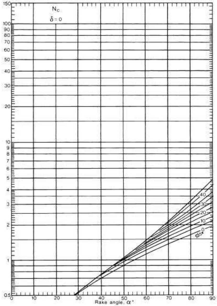
Figure A. 3: Chart of N_c for \delta=0 (Hettiaratchi,1974)
